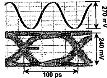
Fig. 15. Recovered 10 GHz clock and 10 Gb/s data from the 1:4 demultiplexer.
