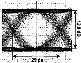
Fig. 8. 40 Gb/s optical output from the lithium niobate modulator after 0 km
