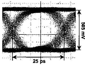
Fig. 12. 40 Gb/s single-ended output from the receiver module.
