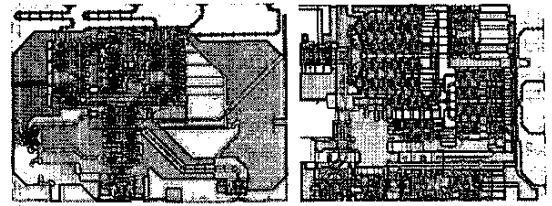
Fig. 3. Micrograph of the 40 Gb/s 4:1 multiplexer and 1:4 demultiplexer (3.3 mm x 3.3 mm each).
