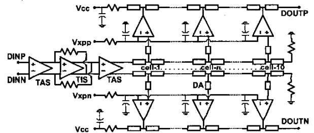
Fig. 5. Schematic of the 40 Gb/s differential modulator driver.
