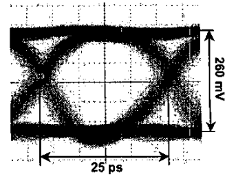
Fig. 4. 40 Gb/s output from the 4:1 multiplexer
