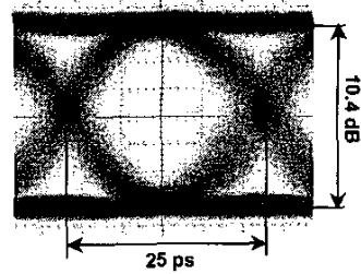
Fig. 10. 40 Gb/s optical output from the EAM after 0 km.
