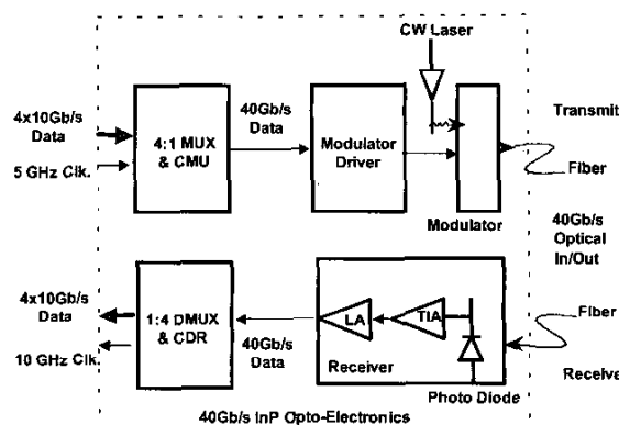
Fig. 1. Block diagram of the 40 Gb/s TDM system.
