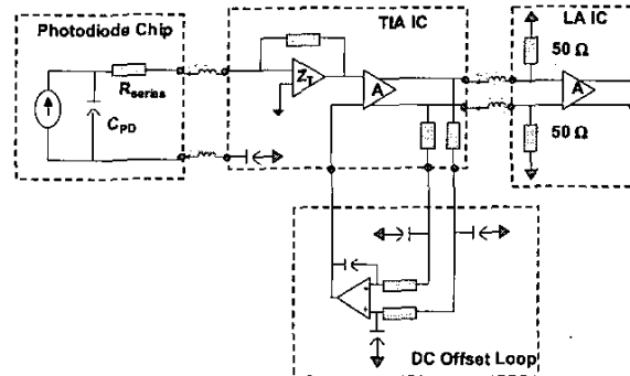
Fig. 11. Schematic of the 40 Gb/s receiver.
